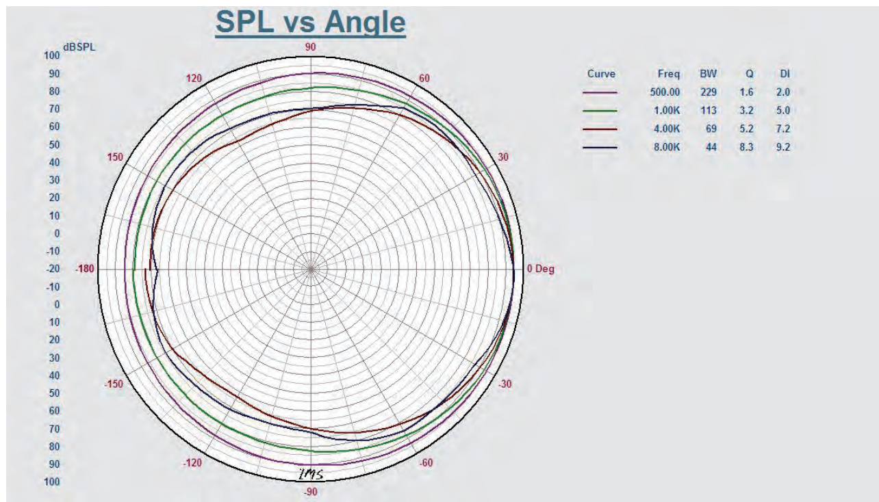
Direction Diagram
