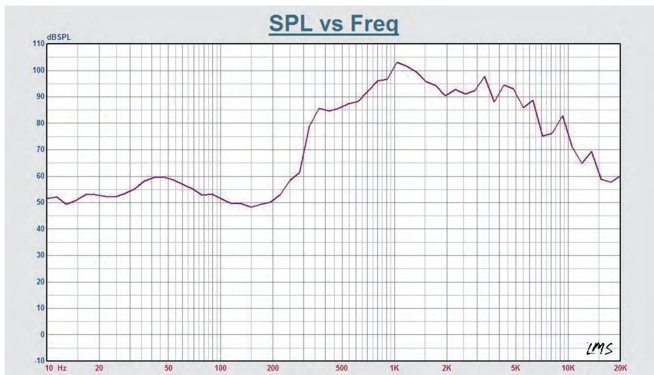
Frequency Response
