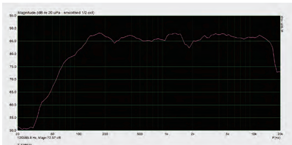
Frequency response
