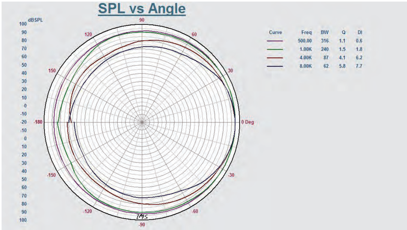
Direction Diagram
