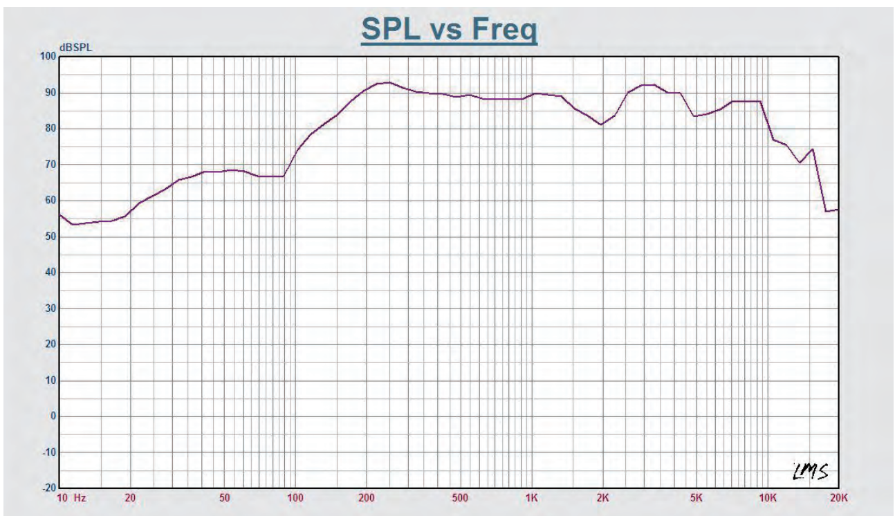
Frequency Response
