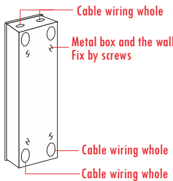
Front panel installation diagram
